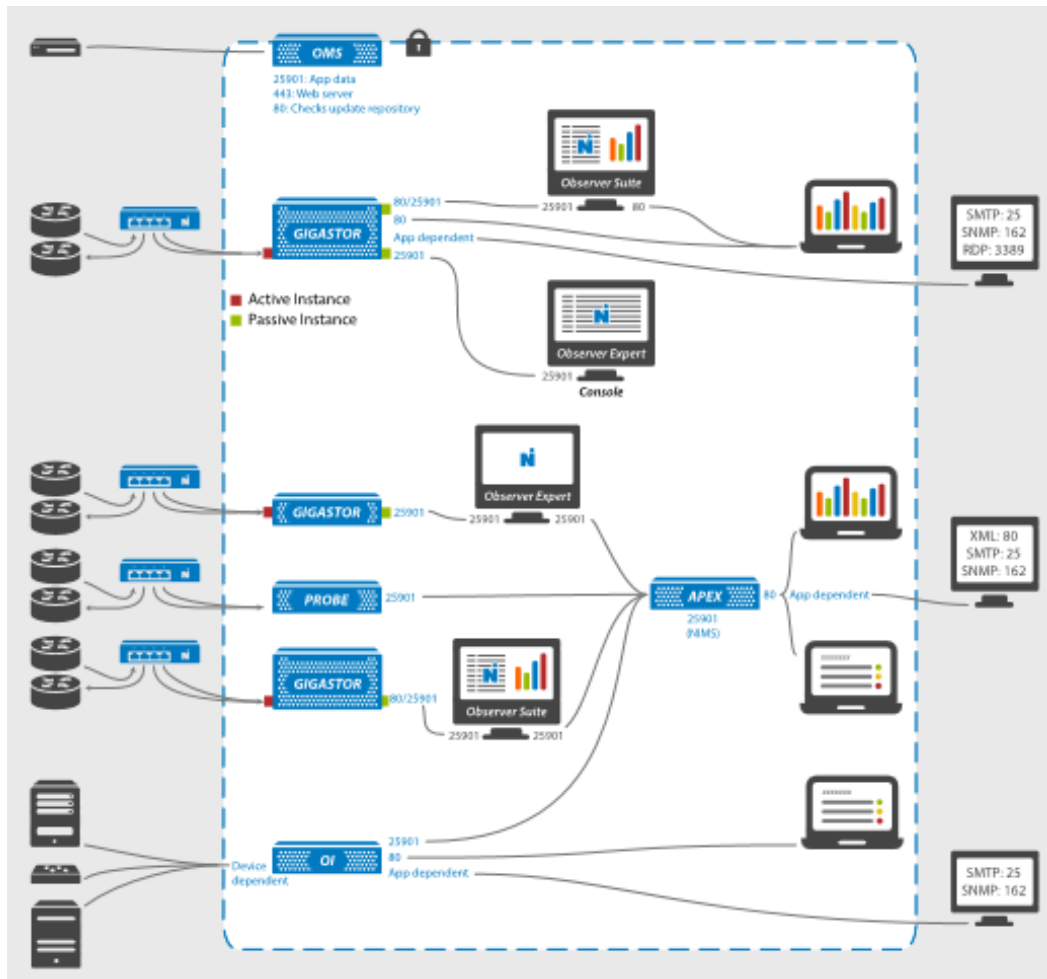
Figure 1: Observer Platform architecture
