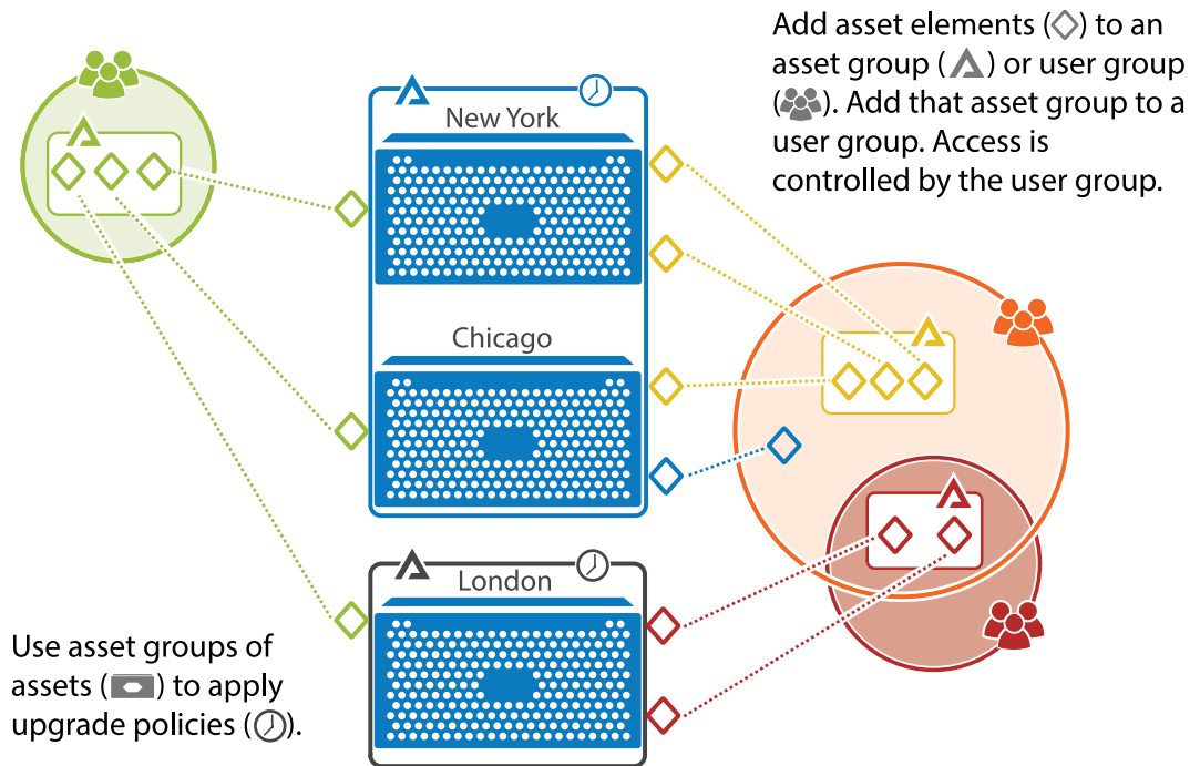
Figure 3: OMS Relationships
