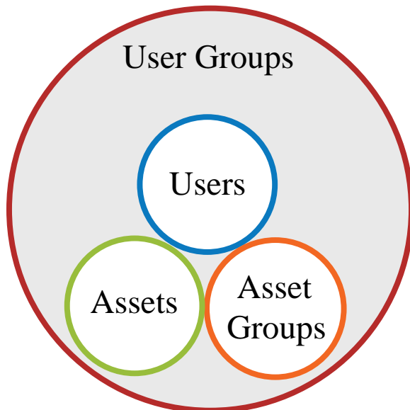
Figure 2: User Groups
